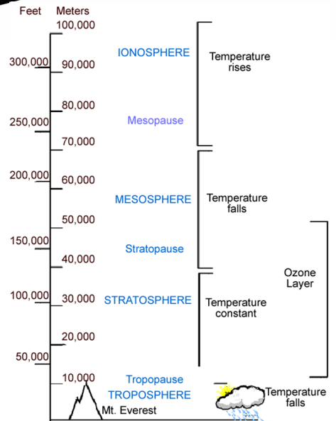
DIVISION OF EARTH'S ATMOSPHERE
