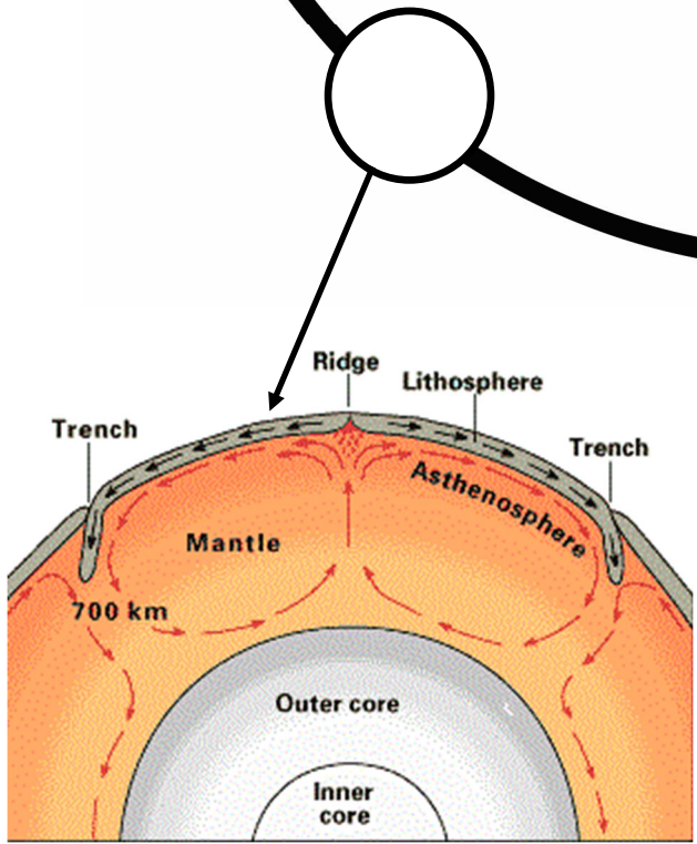
DIVISION OF CRUST AND UPPER MANTLE
