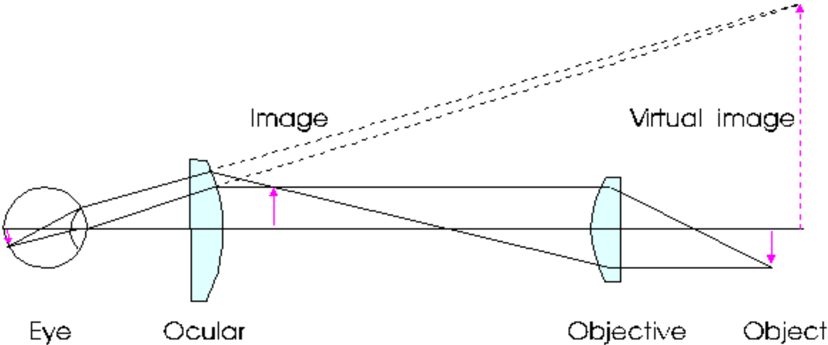
Image Formation in the Compound Microscope.
