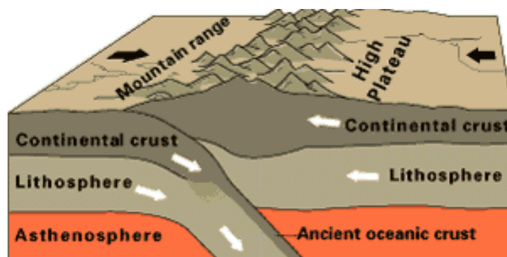
Continental-continental convergence
