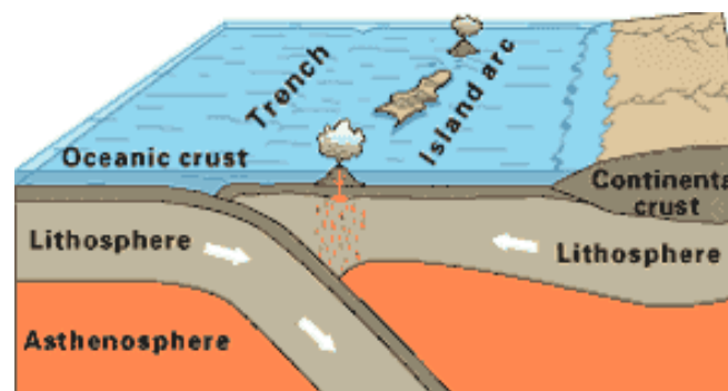
Oceanic-oceanic convergence
