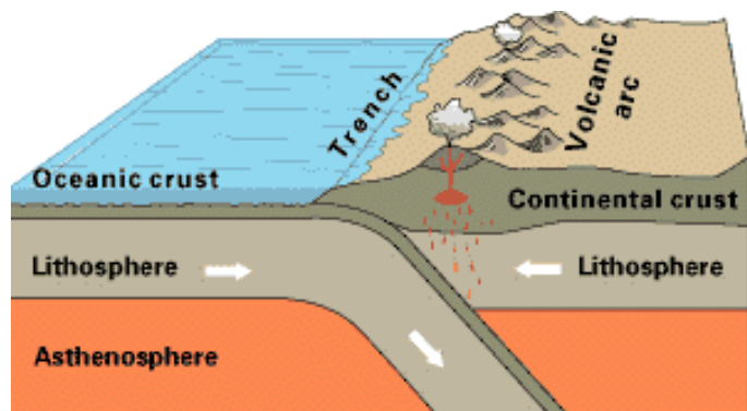
Oceanic-continental convergence
