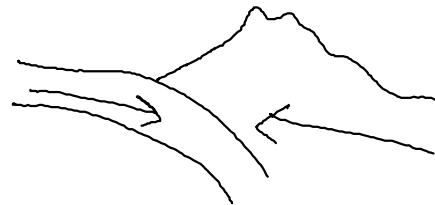
metamorphic
