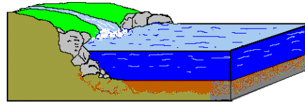
sedimentary
