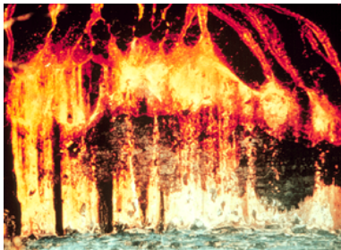
igneous
