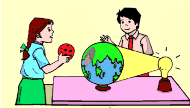
Lunar Eclipse, Earth between Sun and Moon
